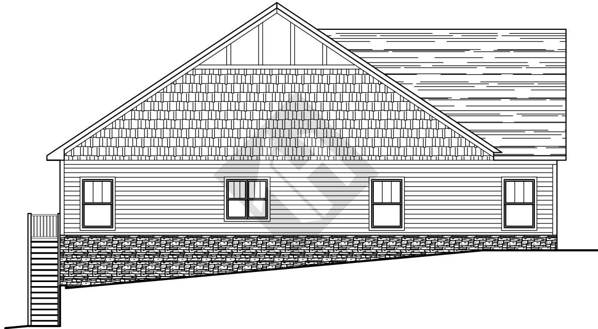
Left Elevation
