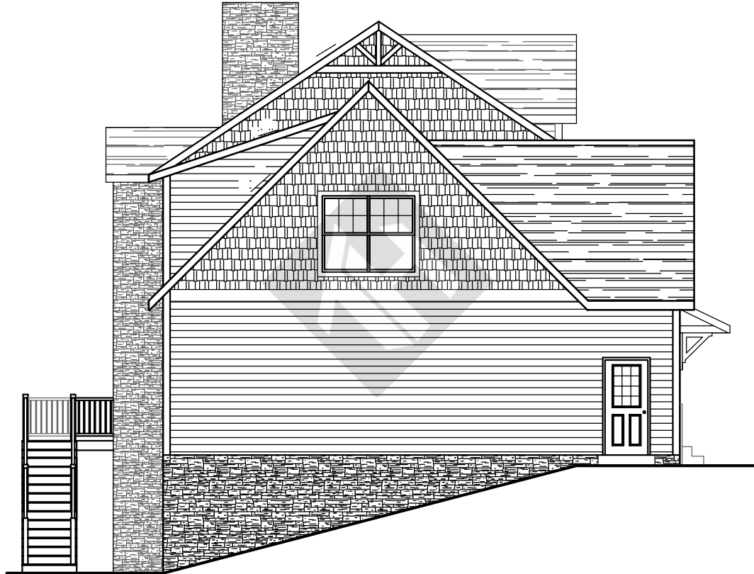
Left Elevation
