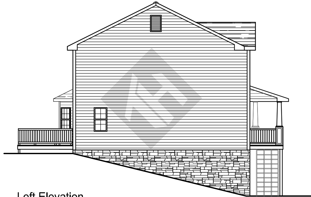
Left Elevation
