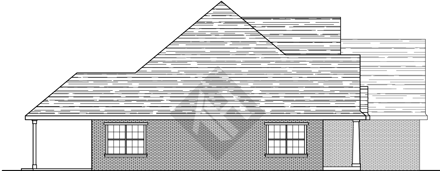
Left Elevation
