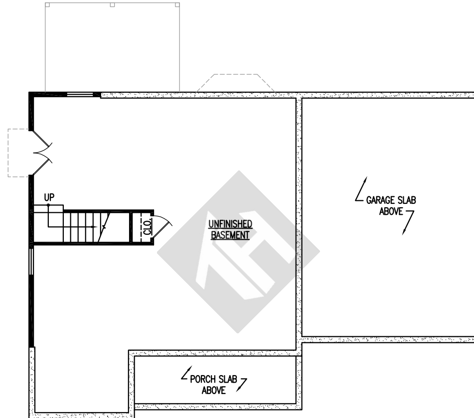
Lower Level Floor Plan
