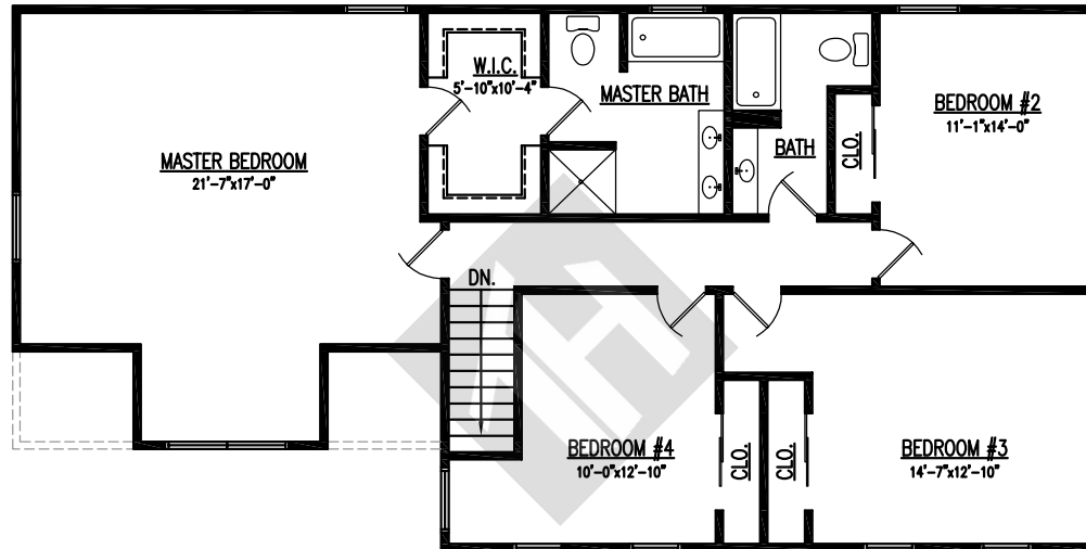
Upper Level Floor Plan
