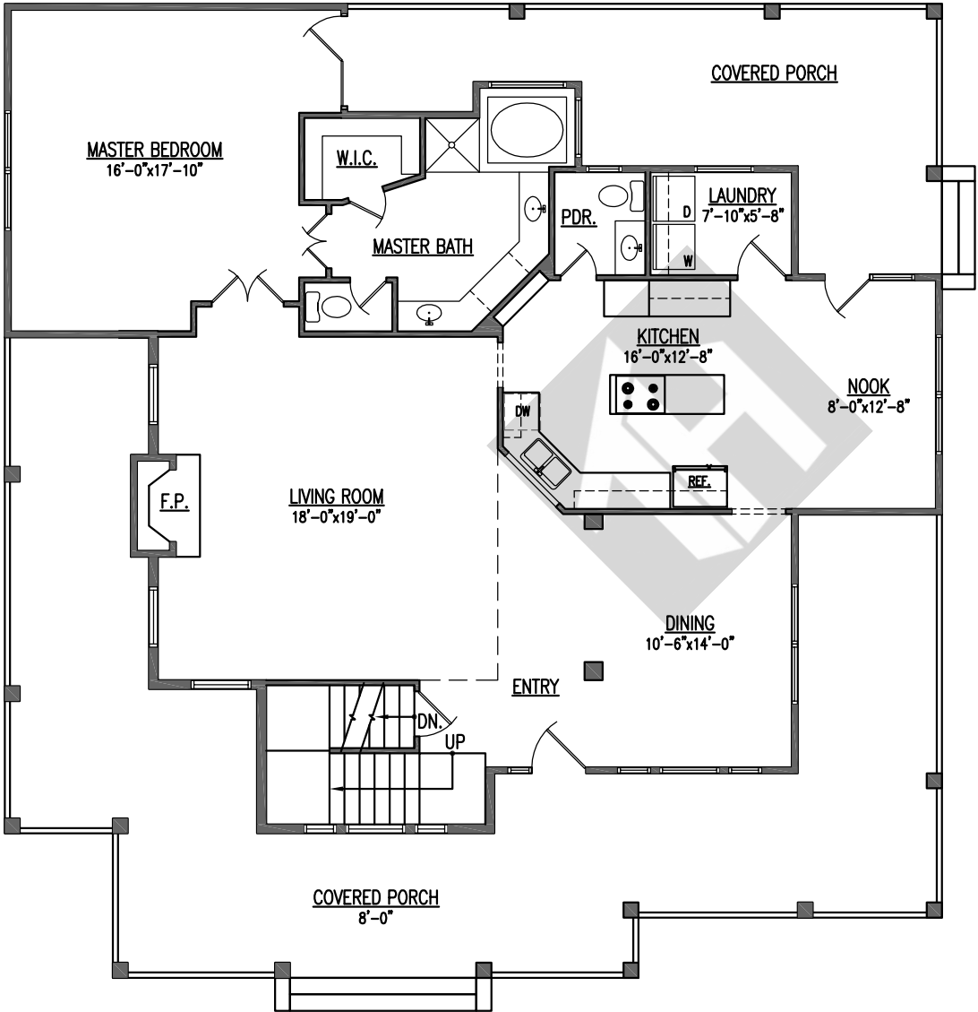
Main Level Floor Plan
