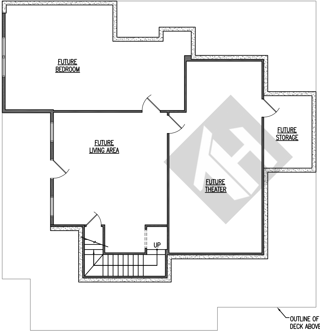
Basement Level Floor Plan
