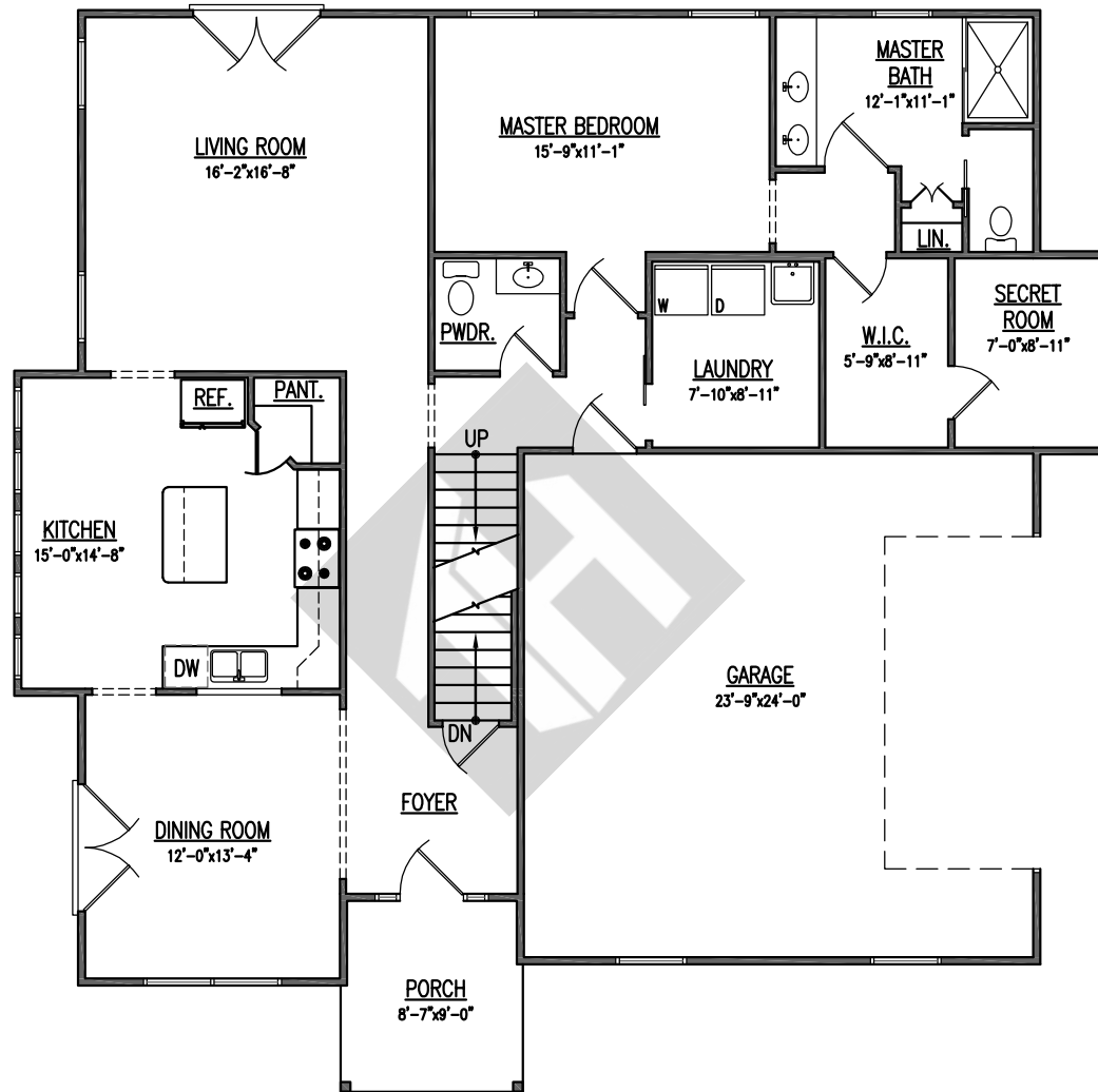
Main Level Floor Plan
