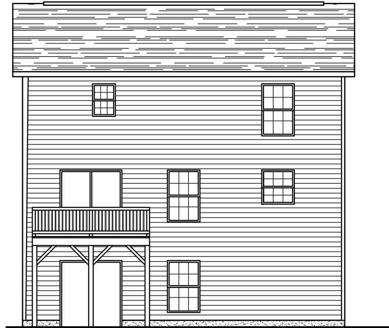
Rear Elevation
