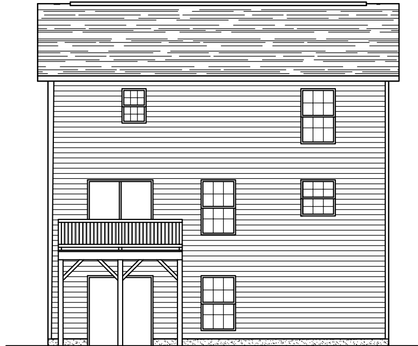
Rear Elevation
