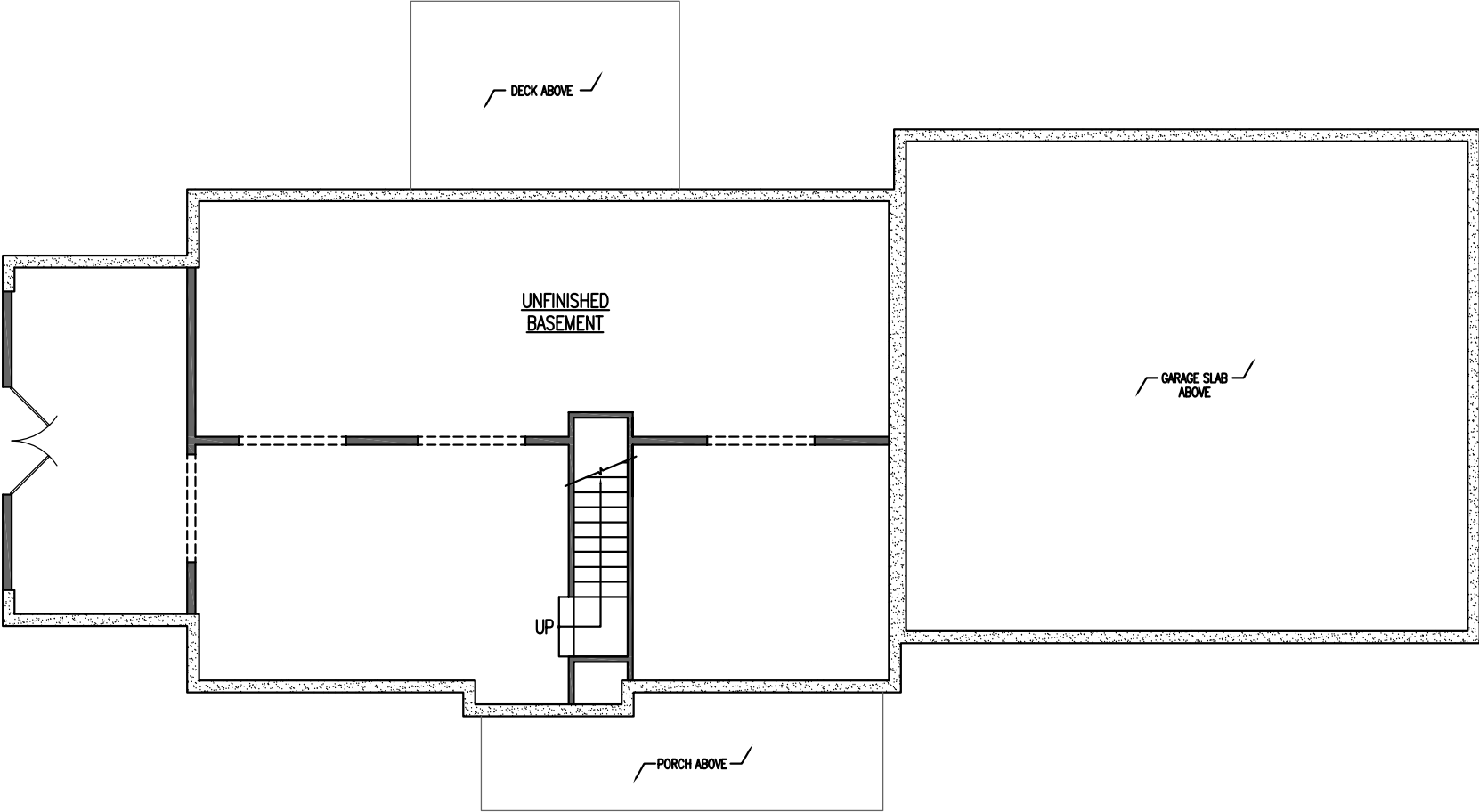
Basement Level Floor Plan
