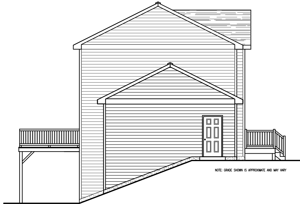
Left Elevation
