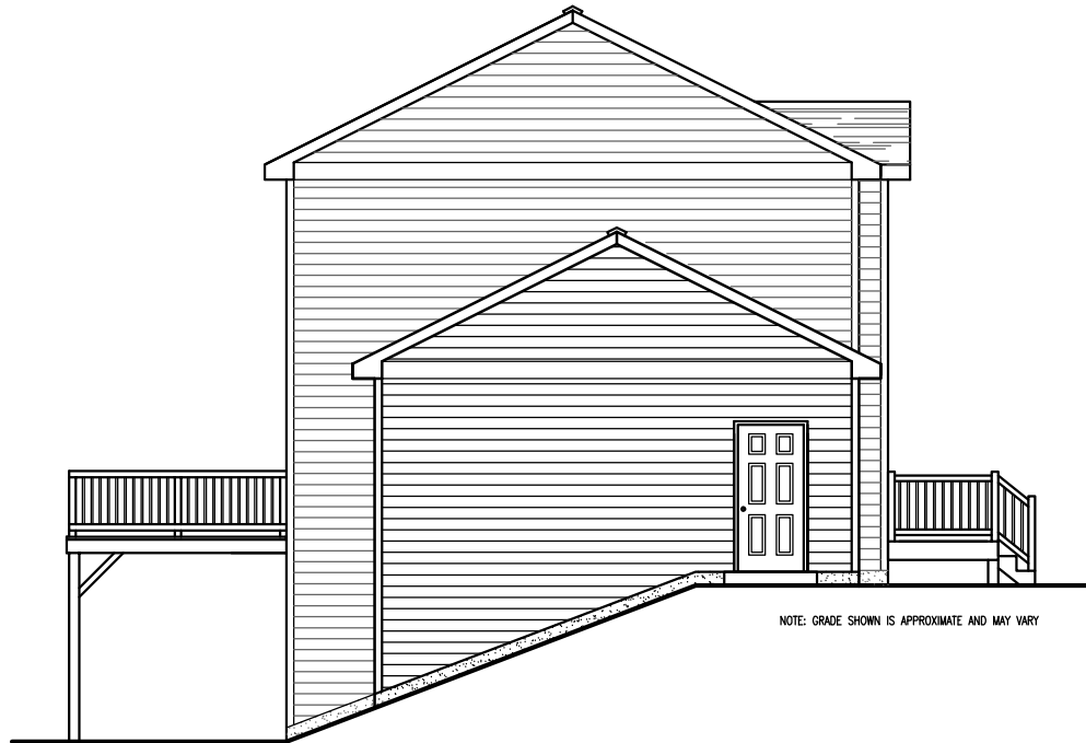
Left Elevation
