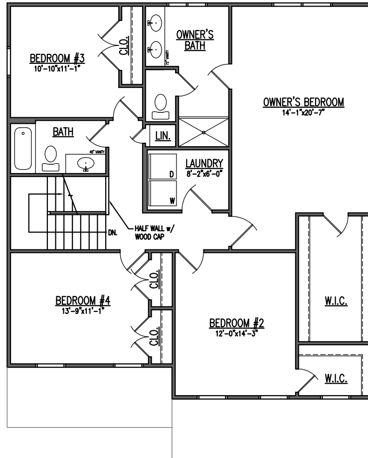
Upper Level Floor Plan
