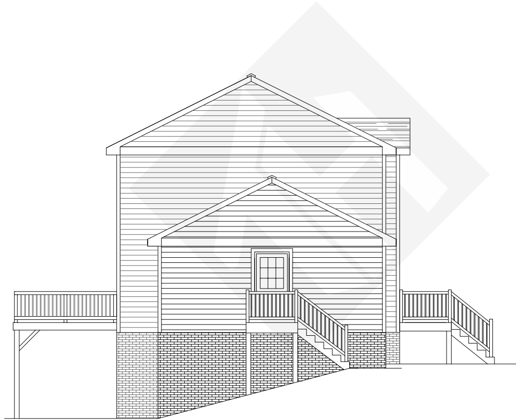
Left Elevation
