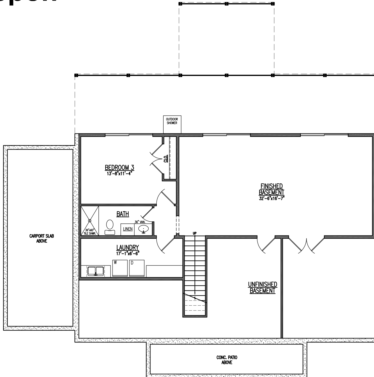
Basement Level Floor Plan
