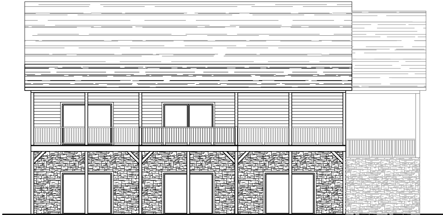
Rear Elevation
