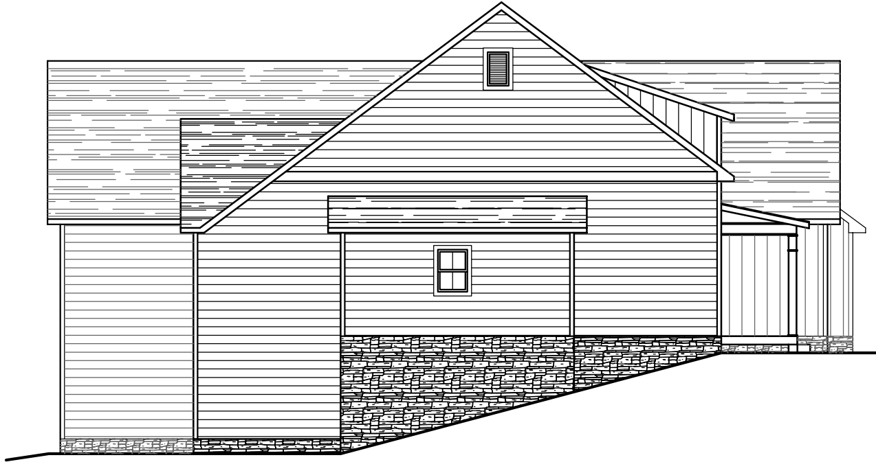
Left Elevation
