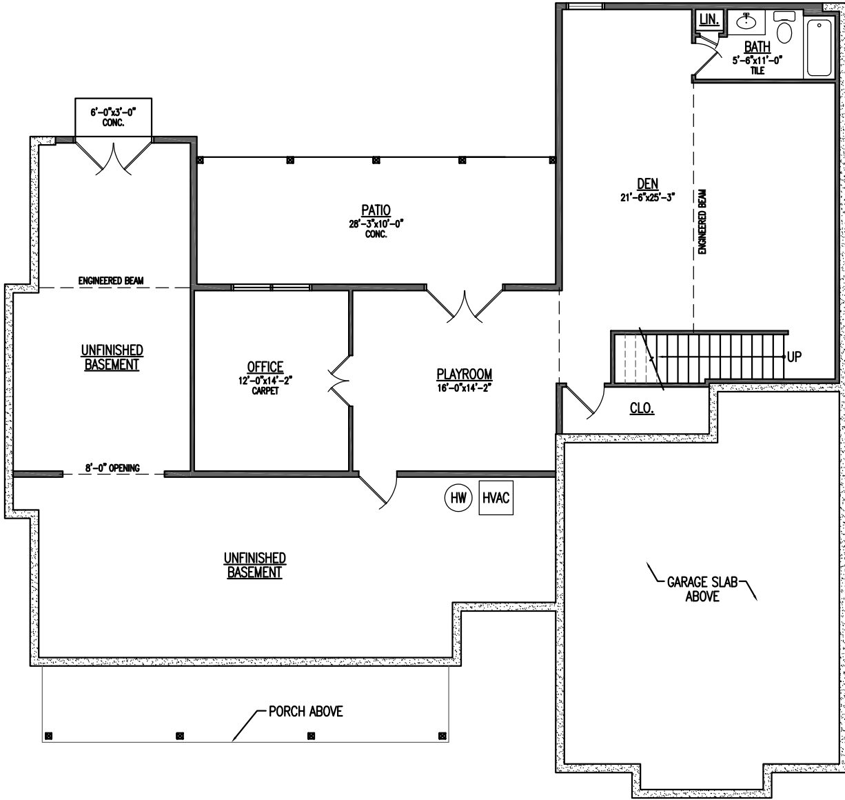
Lower Level Floor Plan
