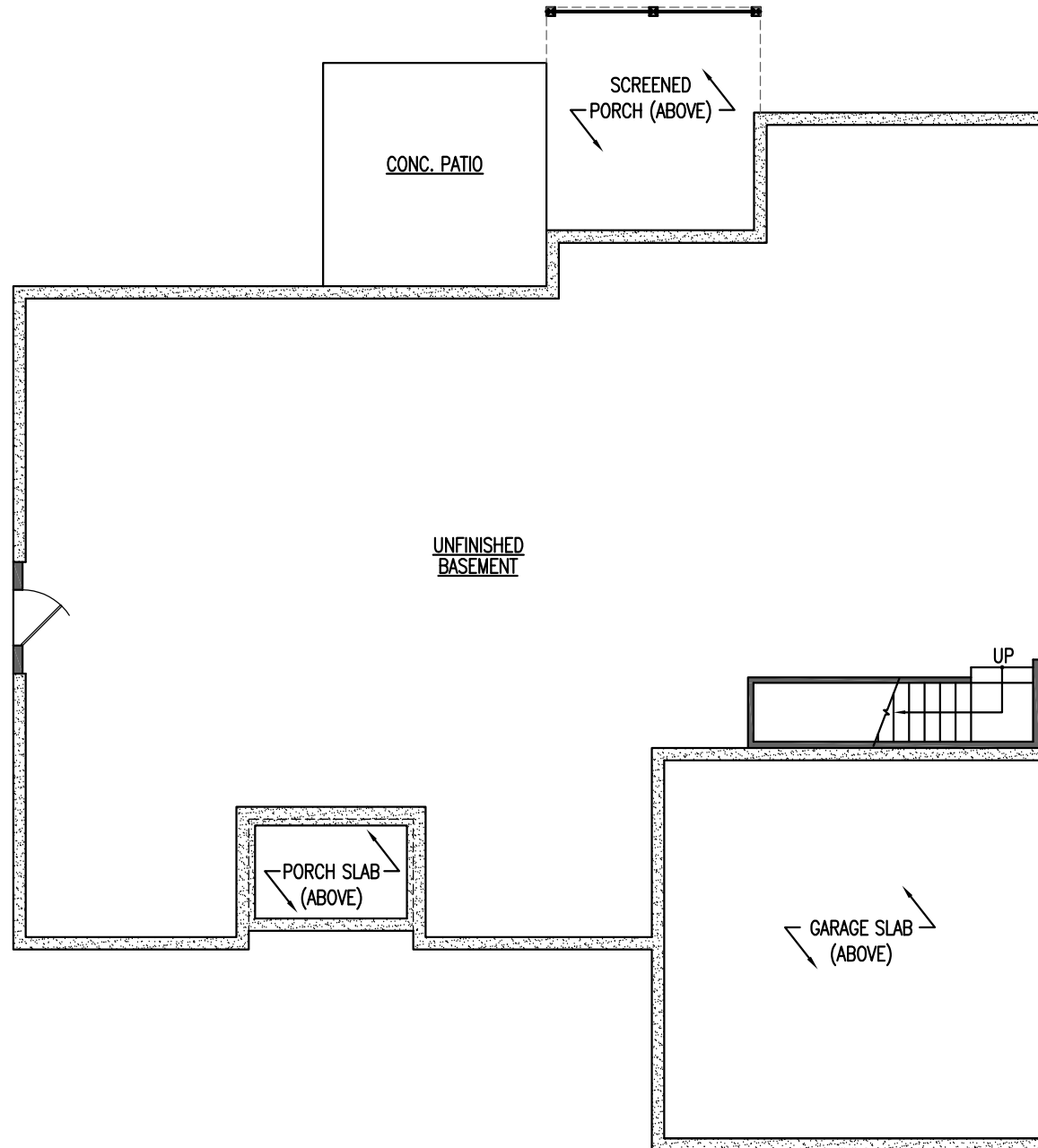
Basement Level Floor Plan
